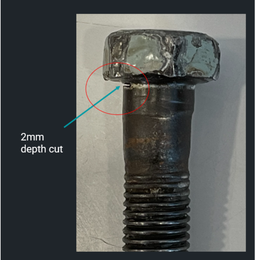
Bolt with a 2mm depth cut to simulate a defect.
